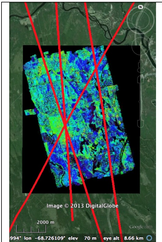
2011 Eco3D SIMPL flight path (red) on Aug. 30, 2011 across Howland forest, Maine G-LiHT canopy height model
