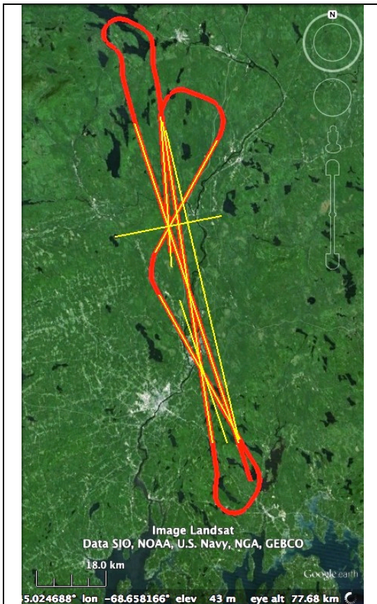
2011 Eco3D SIMPL flight lines (yellow) and flight path (red) on Aug. 30, 2011 at Howland and Penobscot forests, Maine.
