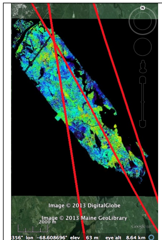
2011 Eco3D SIMPL flight path (red) on Aug. 30, 2011 across Penobscot forest, Maine G-LiHT canopy height model
