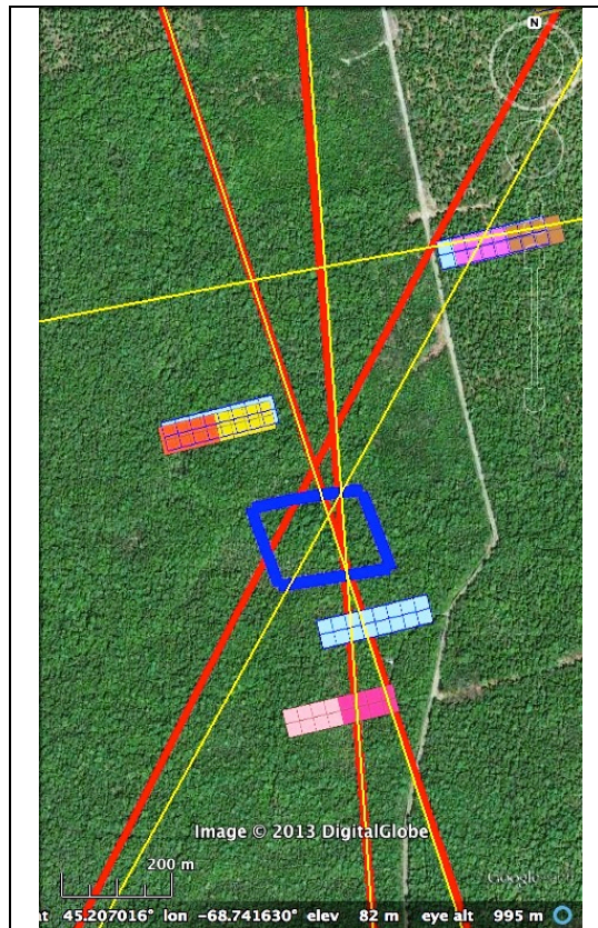
2011 Eco3D SIMPL flight lines (yellow) and flight path (red) on August 30, 2011 across Howland stem map (blue rectangle) and nearby field plots.
